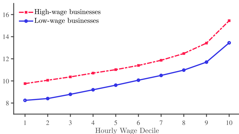
Figure 2: Hourly Wages Within Businesses
