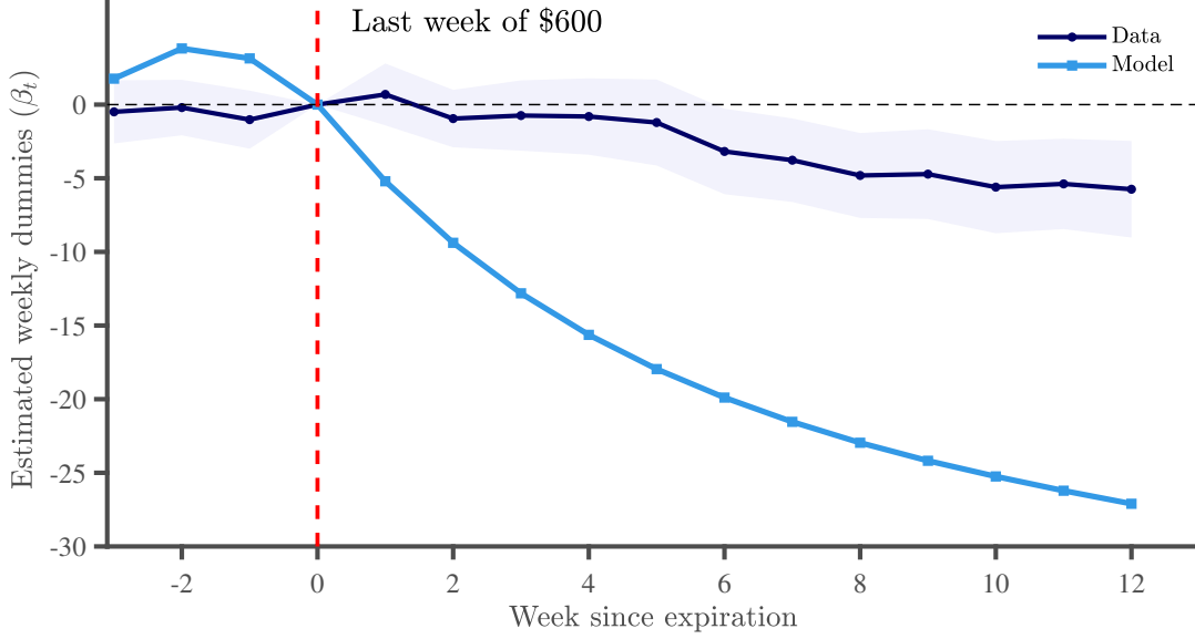
Figure 9: Effects of $600 Expiration on Employment Recovery: Model vs. Data
